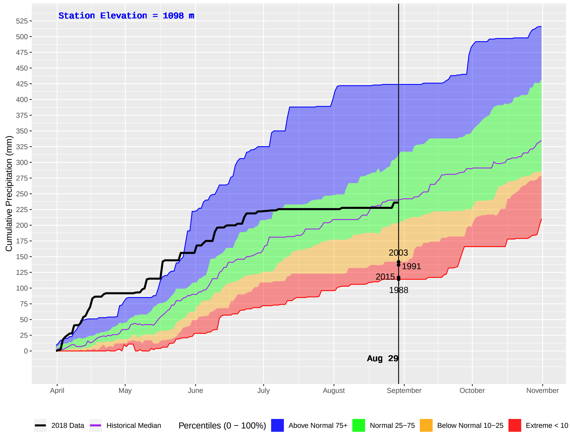
GOATFELL (401) : Historical (1986–2016) and Current (2018) Daily Cumulative Precipitation
